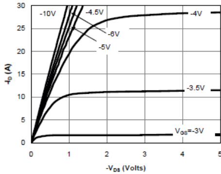
Fig 1: On-Region Characteristics
