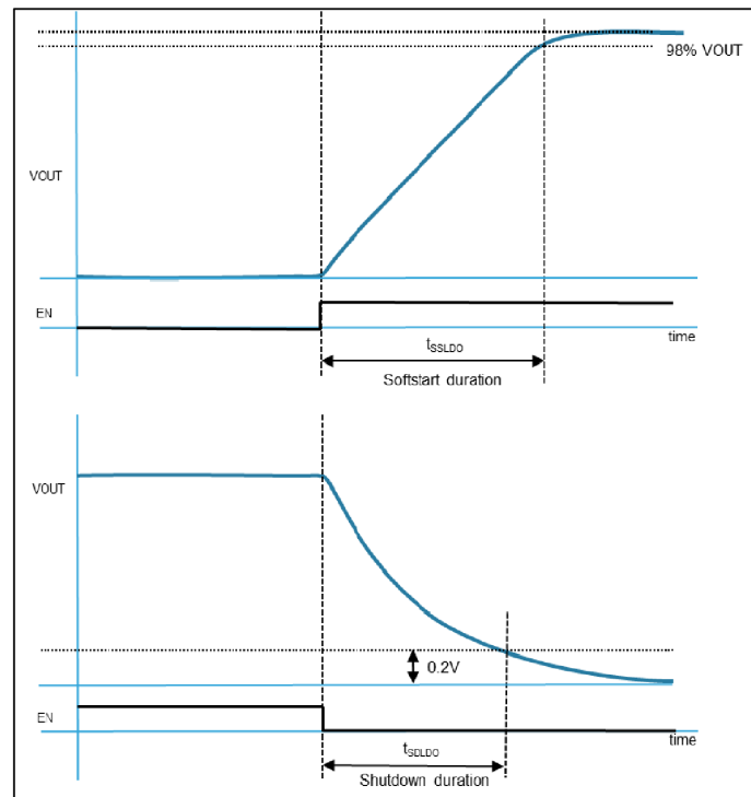
Figure 3. LDO startup/shutdown timings
