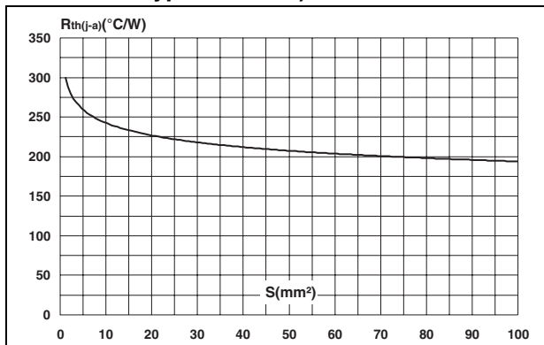
Figure 9. Thermal resistance junction to ambient versus copper surface under each lead (epoxy printed circuit board FR4, Cu = 35 \mu\text{m} , typical values)
