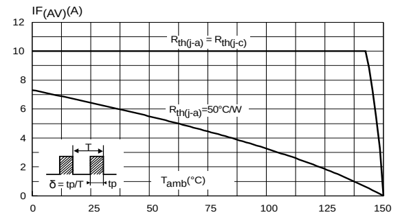
Figure 2: Average forward current versus ambient temperature ( \delta = 0.5 )
