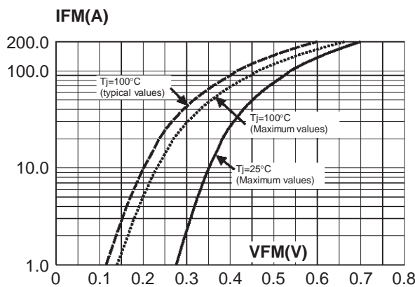
Fig. 7: Forward voltage drop versus forward current (per diode).
