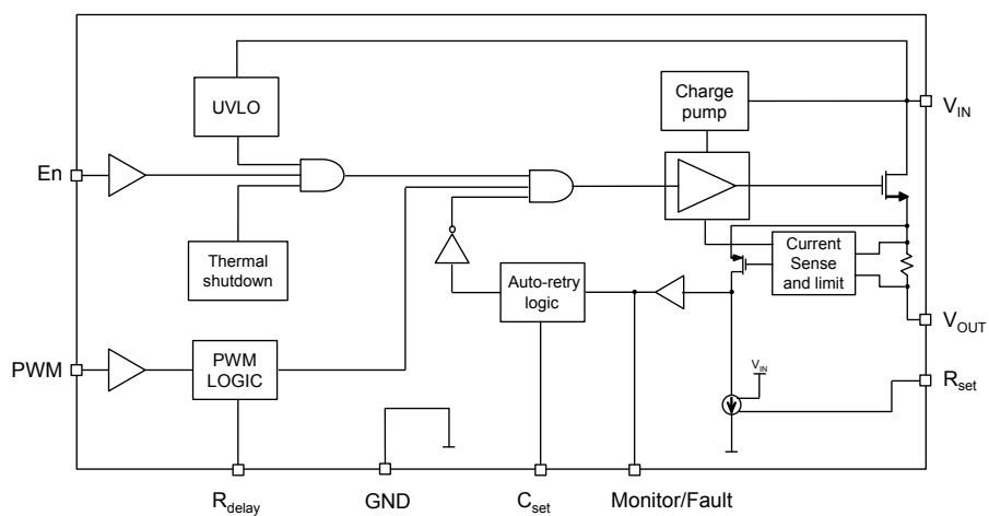
Figure 2. Block diagram
