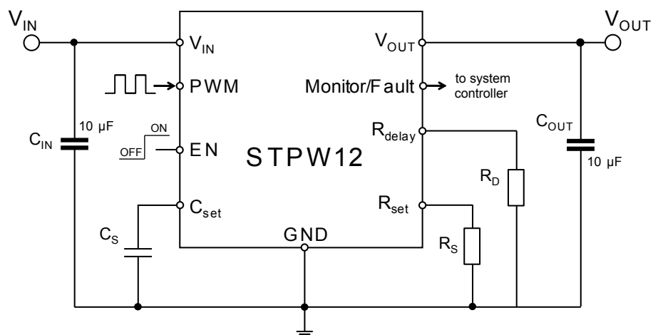
Figure 4. Application circuit
