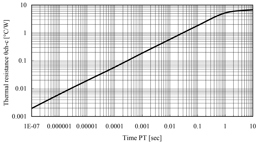
Fig8 MOSFET Transient thermal resistance characteristic
