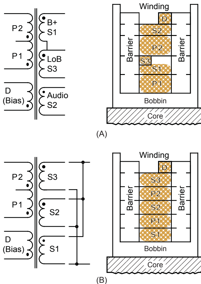
Figure 22. Example of recommended transformers: (A) CRT TV transformer, (B) low output-voltage transformer.
