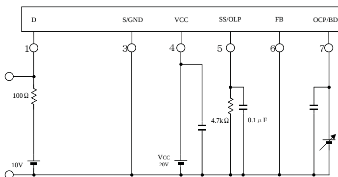
Measurement Circuit 2
