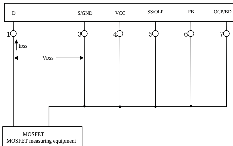
Measurement Circuit 8
