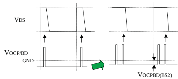
Waveform 2
