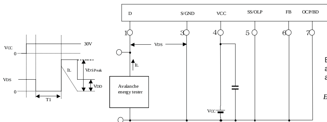
Measurement Circuit 9
