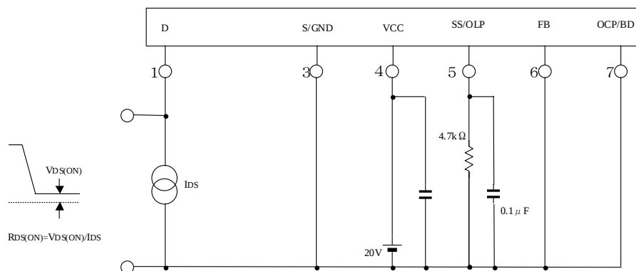
Measurement Circuit 9
