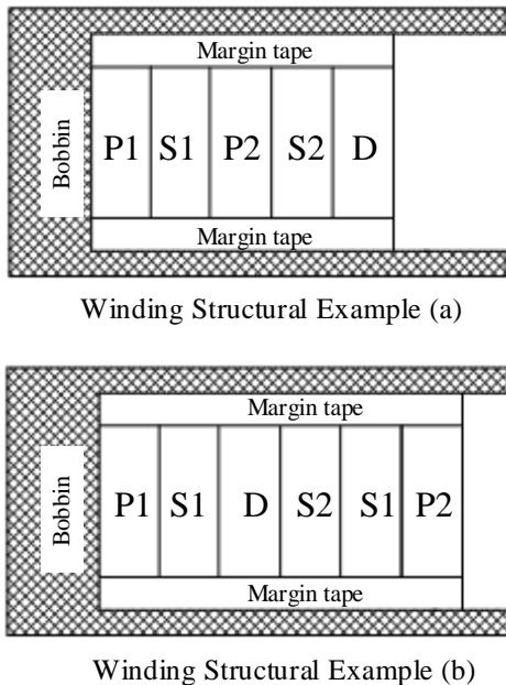
Figure 11-4. Winding Structural Examples
