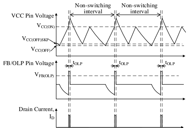
Figure 10-18. OLP Operational Waveforms
