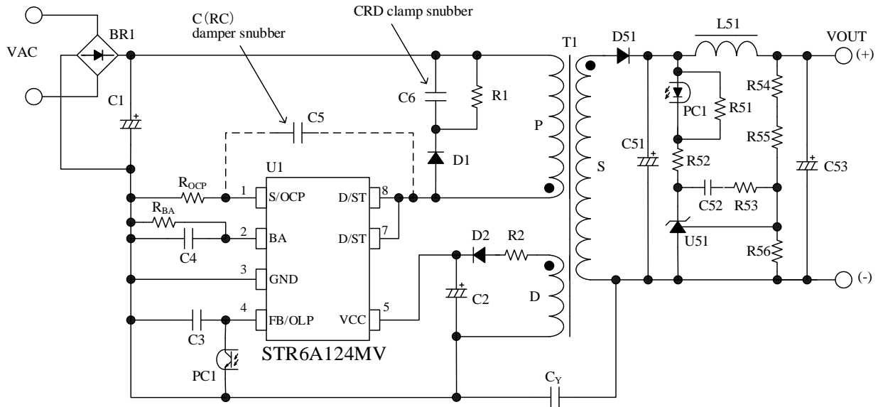
Figure 7-1. Typical Application
