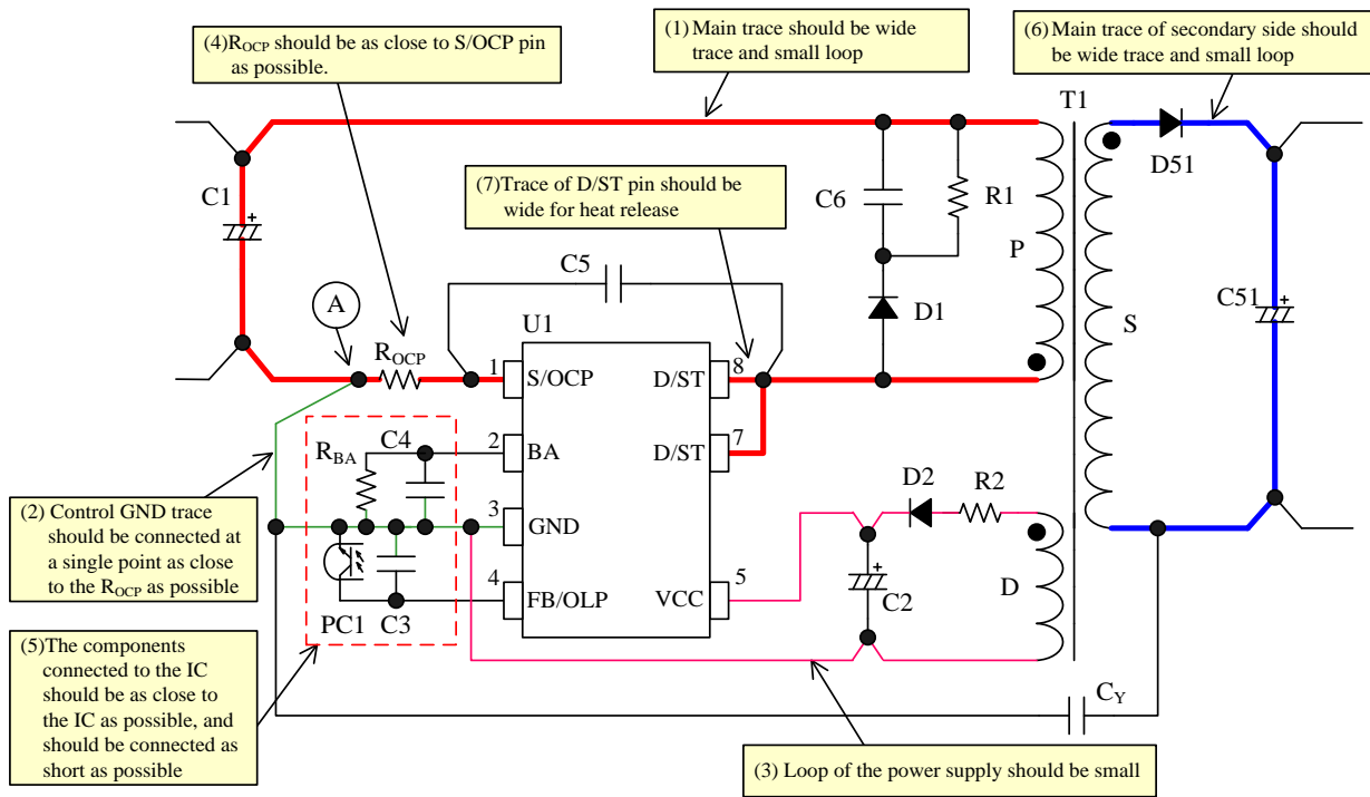
Figure 11-5. Peripheral Circuit Example Around the IC
