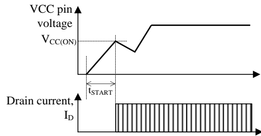
Figure 10-2. Startup Operation
