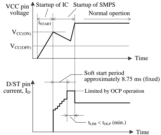
Figure 10-5. VCC and I_D Waveforms during Startup
