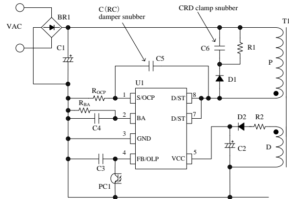
Figure 11-1. The IC Peripheral Circuit
