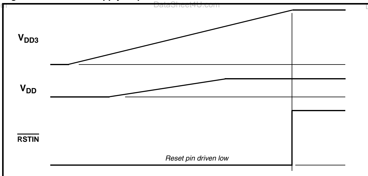
Figure 69. Power-on supply sequence
