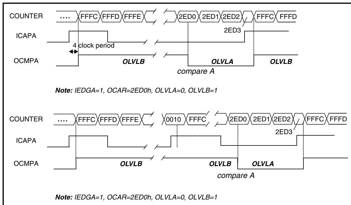
Figure 52. One Pulse Mode Timing
