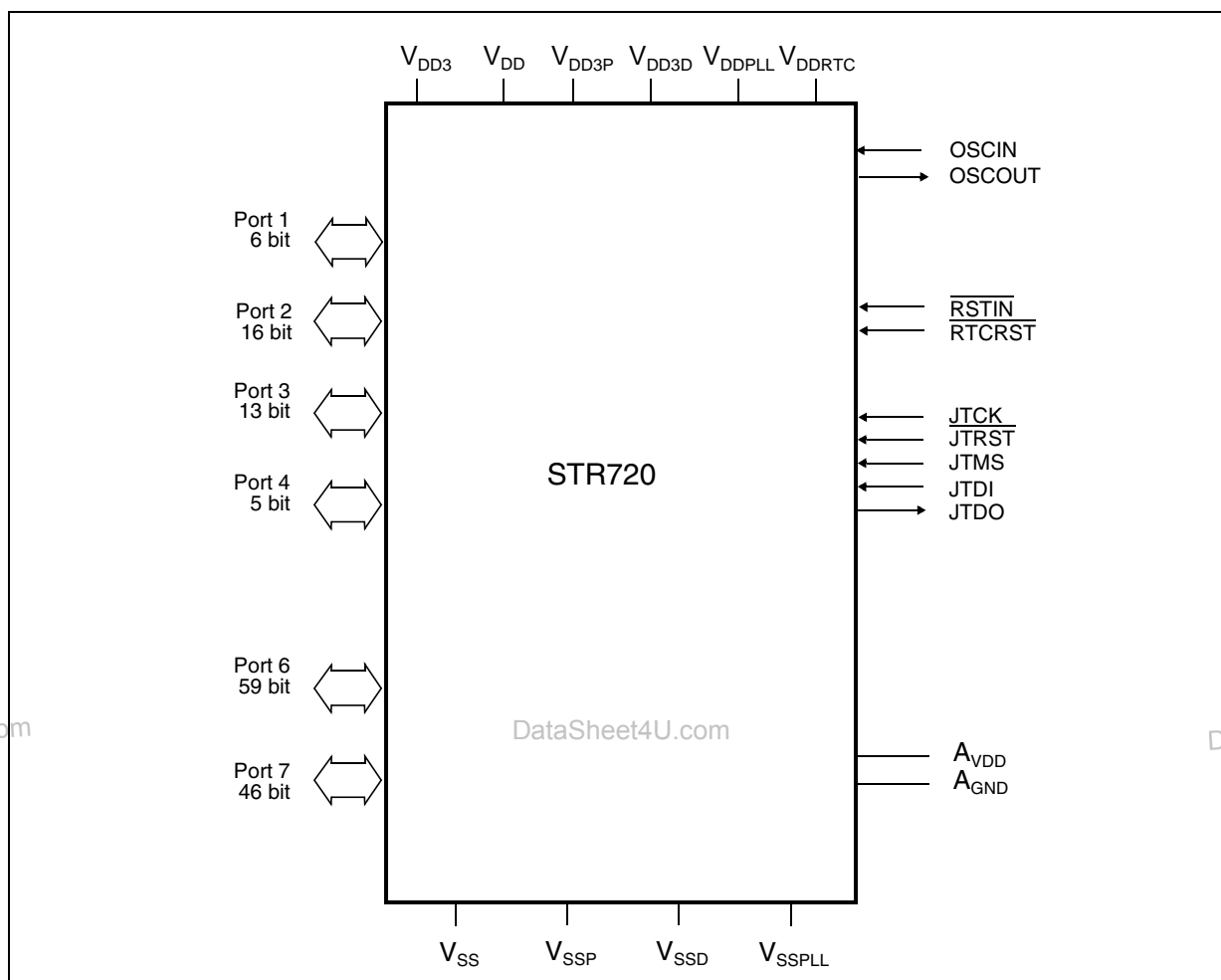
Figure 1. STR720 PQFP Package Logic Symbol
