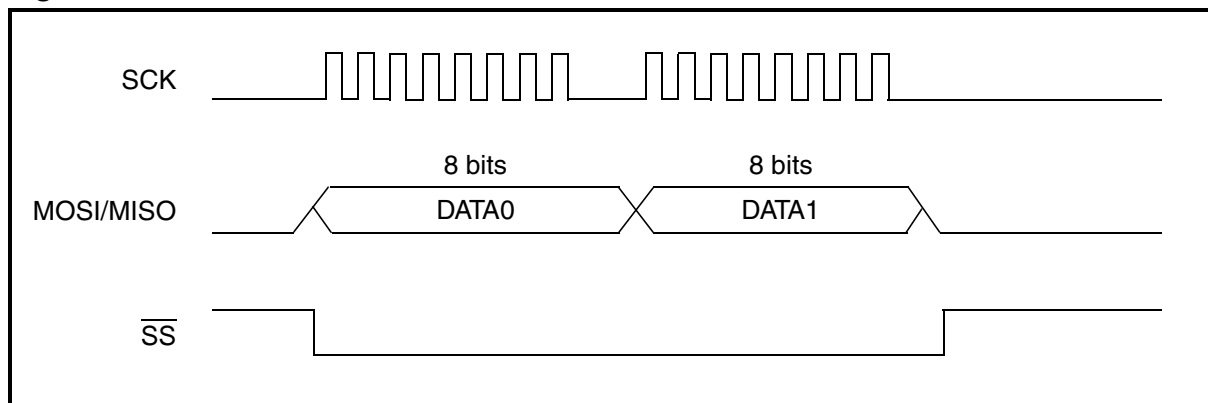
Figure 24. BSPI Bus Transfer
