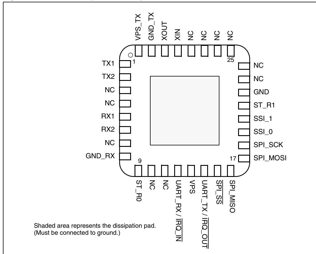
Figure 3. STRFNFCA pinout description
