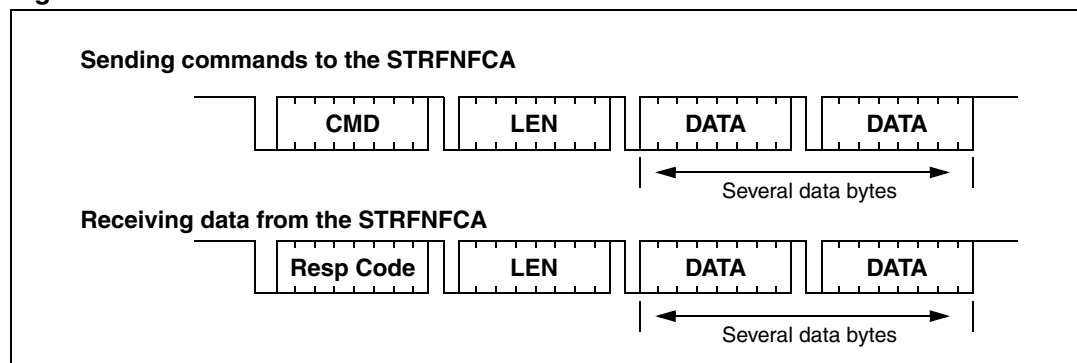
Figure 6. UART communication
