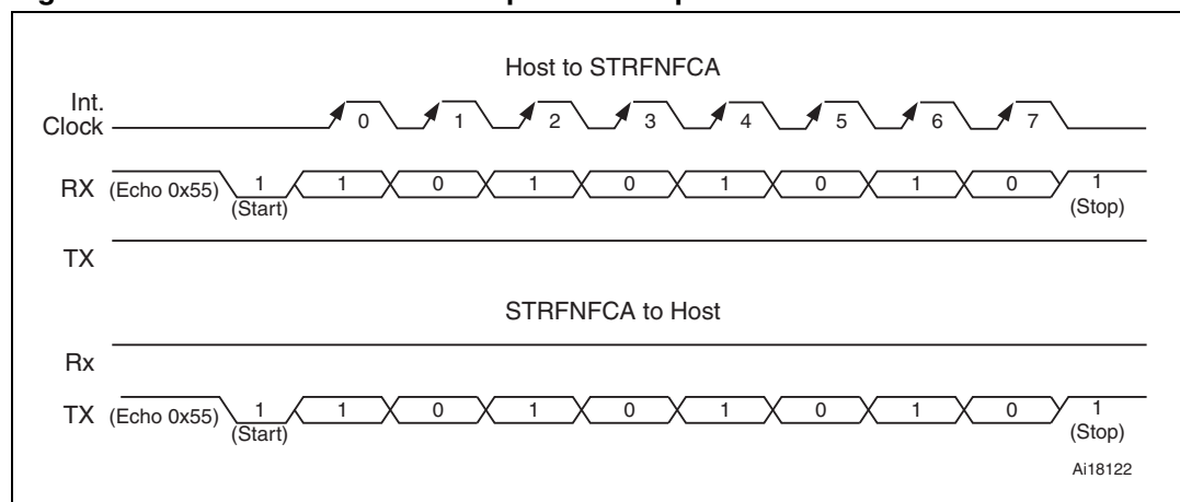
Figure 7. ECHO command and response example
