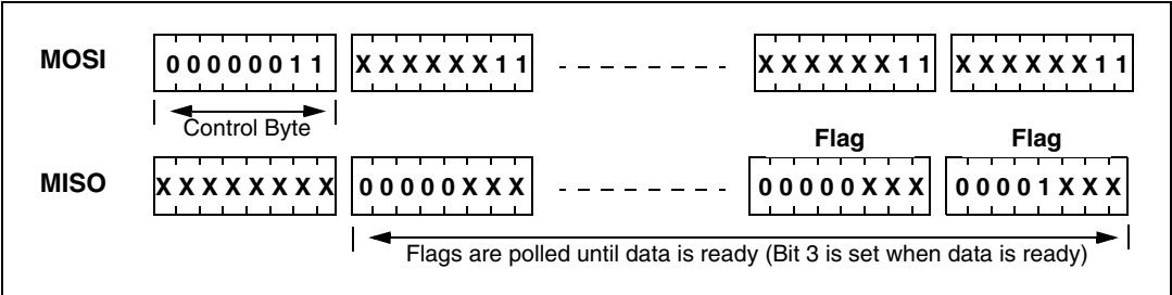
Figure 9. Polling the STRFNFCA until it is ready
