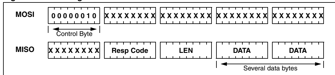
Figure 10. Reading data from STRFNFCA
