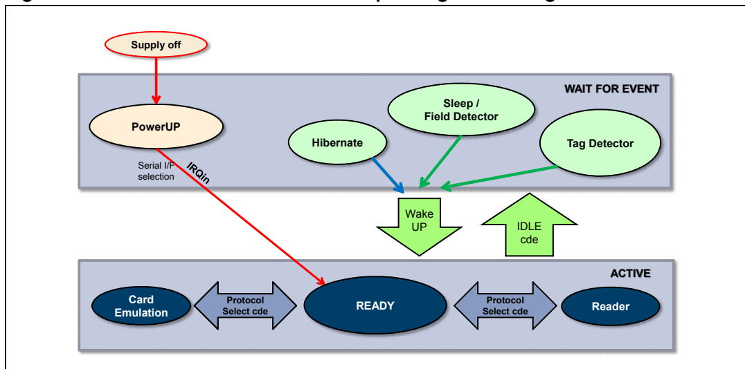
Figure 4. STRFNFCA initialization and operating state change
