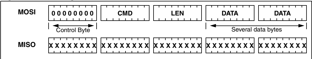
Figure 8. Sending command to STRFNFCA
