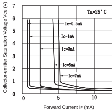
STS710 (Optocoupler Portion)
