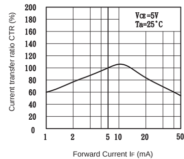
STS710 (Optocoupler Portion)
