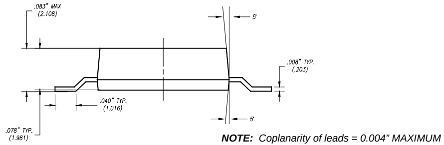
END VIEW
