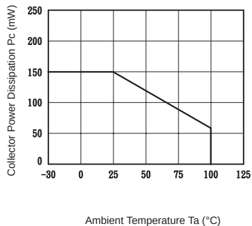
STS710 (Optocoupler Portion)
