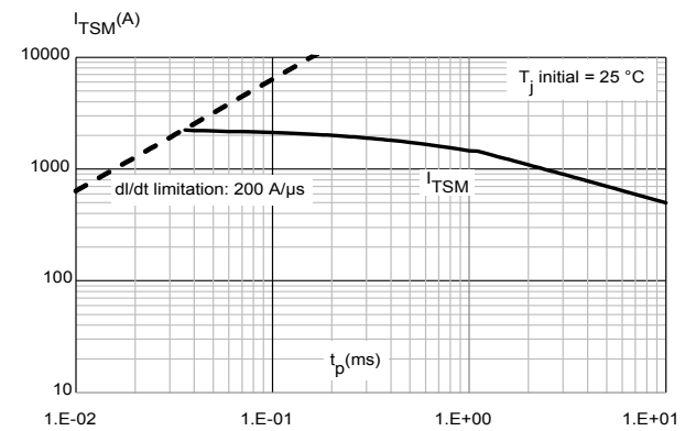
Figure 12. SCR non repetitive surge peak on-state current for a sinusoidal pulse ( t_p < 10 ms), V_r = 0 V
