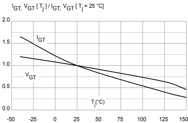
Figure 9. SCR relative variation of gate trigger current and gate trigger voltage versus junction temperature (typical values)
