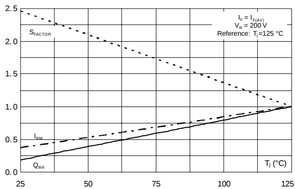
Figure 7: Relative variation of dynamic parameters versus junction temperature
