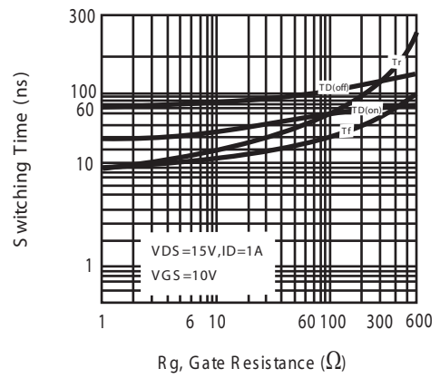
Figure 12. switching characteristics
