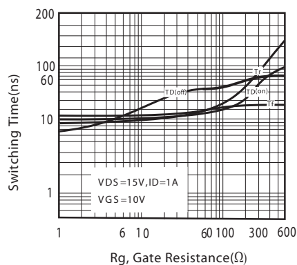
Figure 11. switching characteristics
