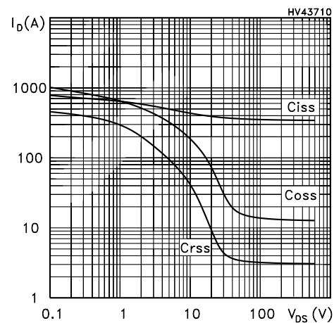
Figure 10. Capacitance variations
