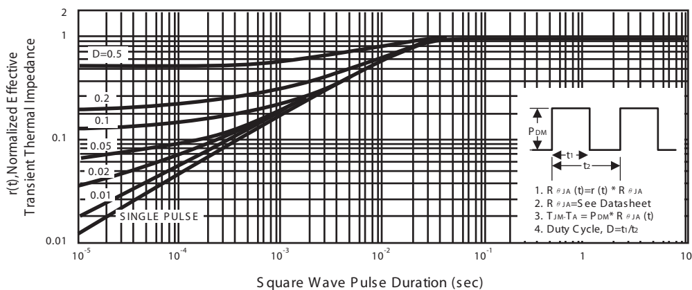
Figure 14. Normalized Thermal Transient Impedance Curve www.DataSheet4U.com
