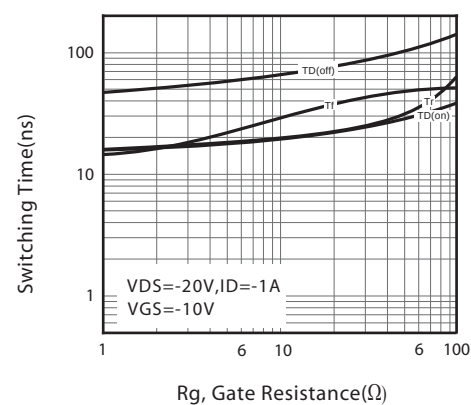
Figure 11. switching characteristics
