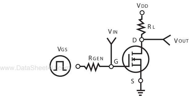
Figure 13. Switching Test Circuit
