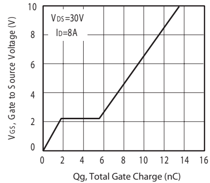
Figure 10. Gate Charge
