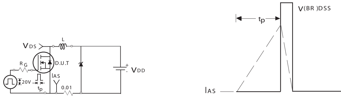
Unclamped Inductive Test Circuit
