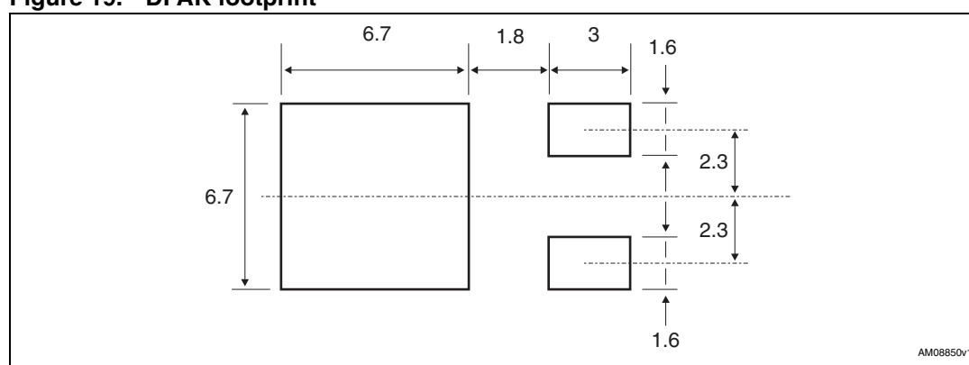
Figure 19. DPAK footprint (a)
