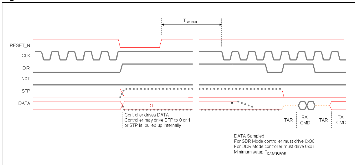
Figure 9. RESETn behavior
