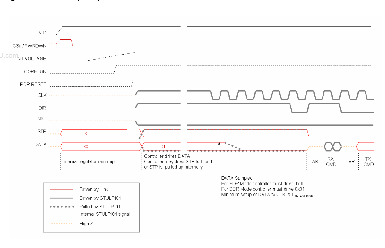
Figure 8. Start-up sequence
