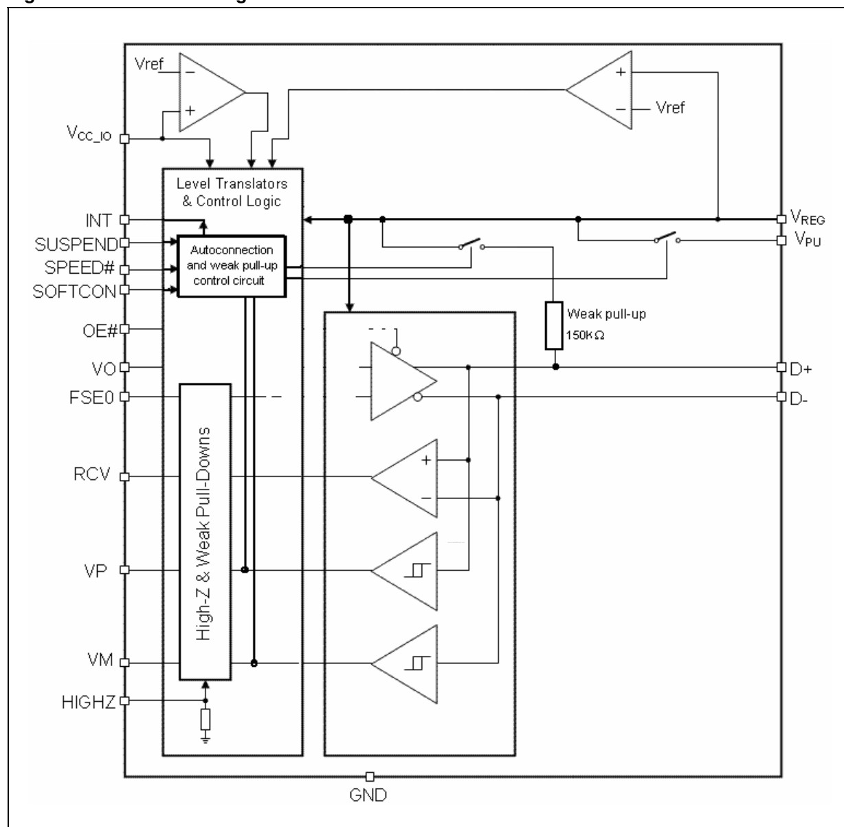
Figure 5. Functional diagram
