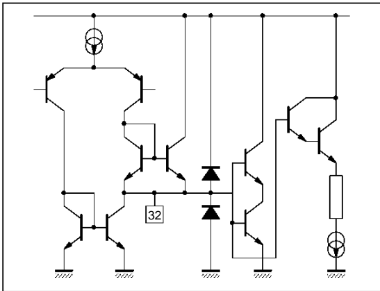
Figure 14 : Pin 32 (CKP)
