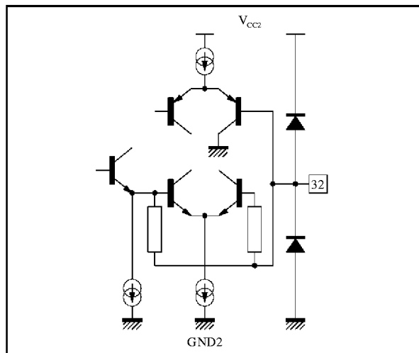
Figure 25 : Pin 32 - SXTL
