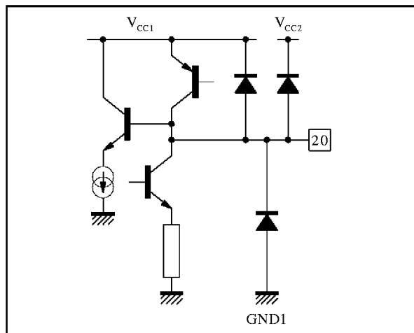
Figure 19 : Pin 20 - Y/CVBS
