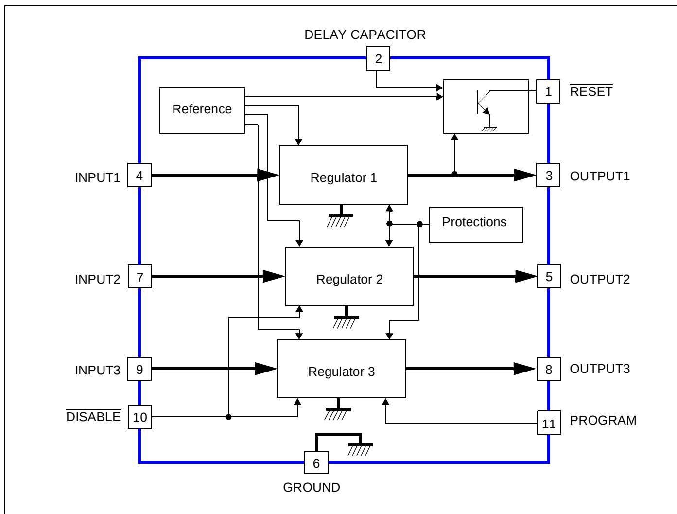
Figure 1: STV8163 Block Diagram
