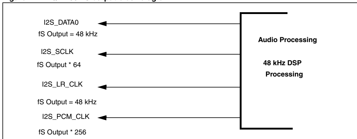
Figure 22. TQFP 80 I 2 S output block diagram
