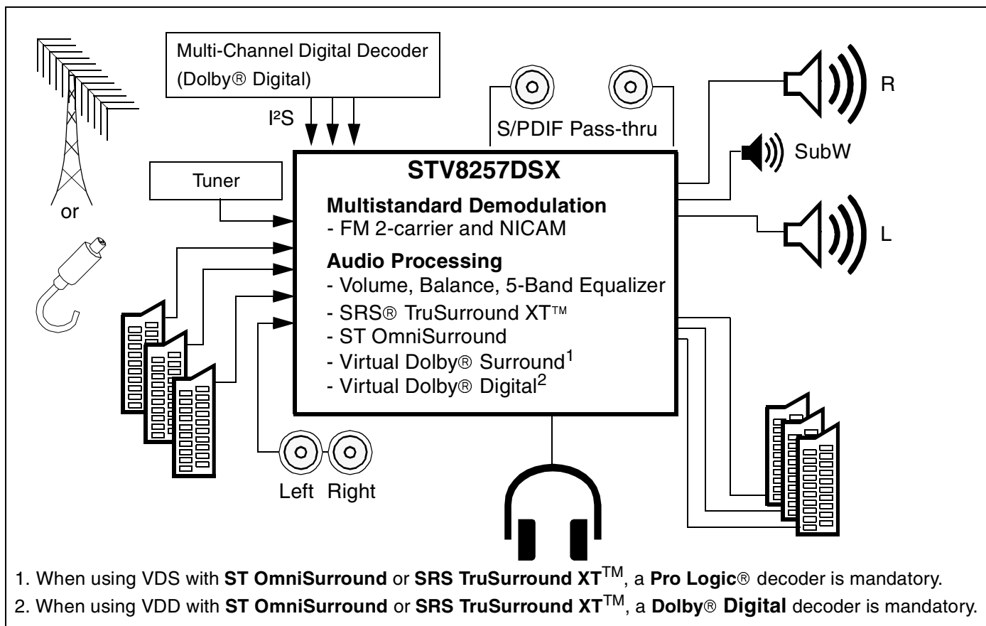
Figure 4: STV8257 Typical Application (Digital: Virtual Sound) www.DataSheet4U.com
