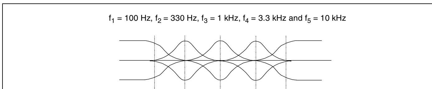
Figure 19: Equalizer
