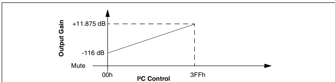
Figure 20: Volume Control
