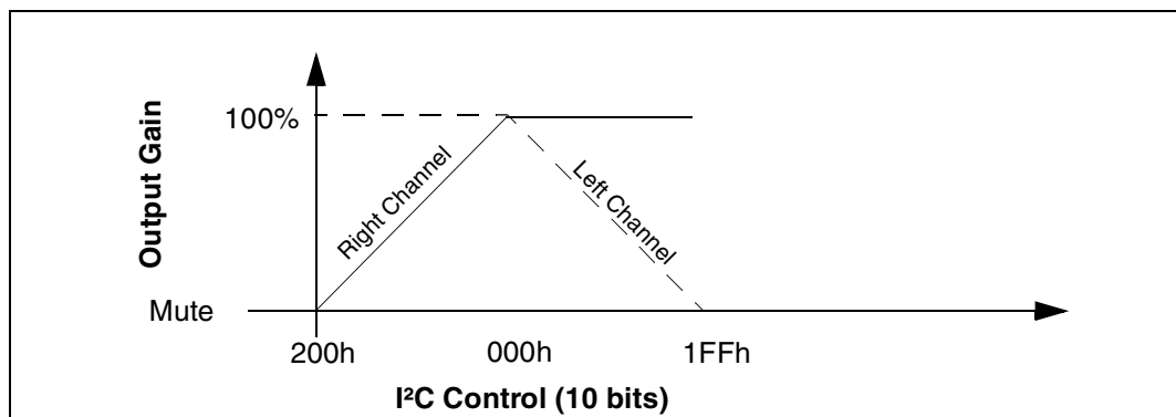
Figure 21: Differential Balance
