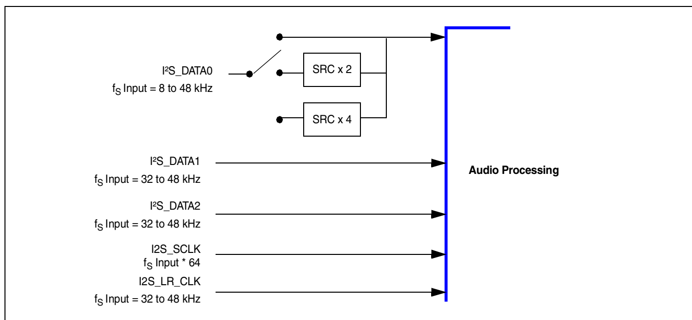
Figure 26: I 2 S Block Diagram
