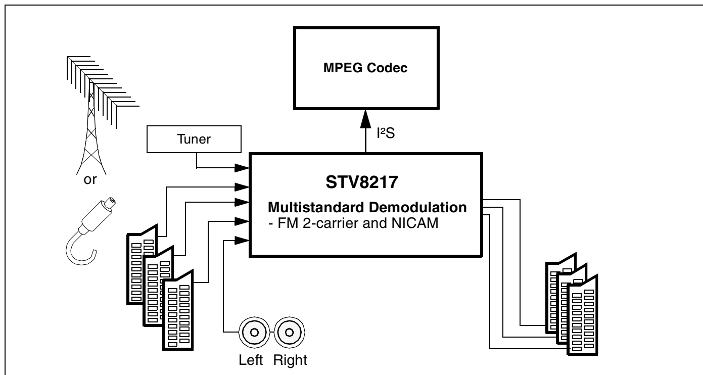
Figure 6: STV8217 Typical Application (Digital Recorder)
