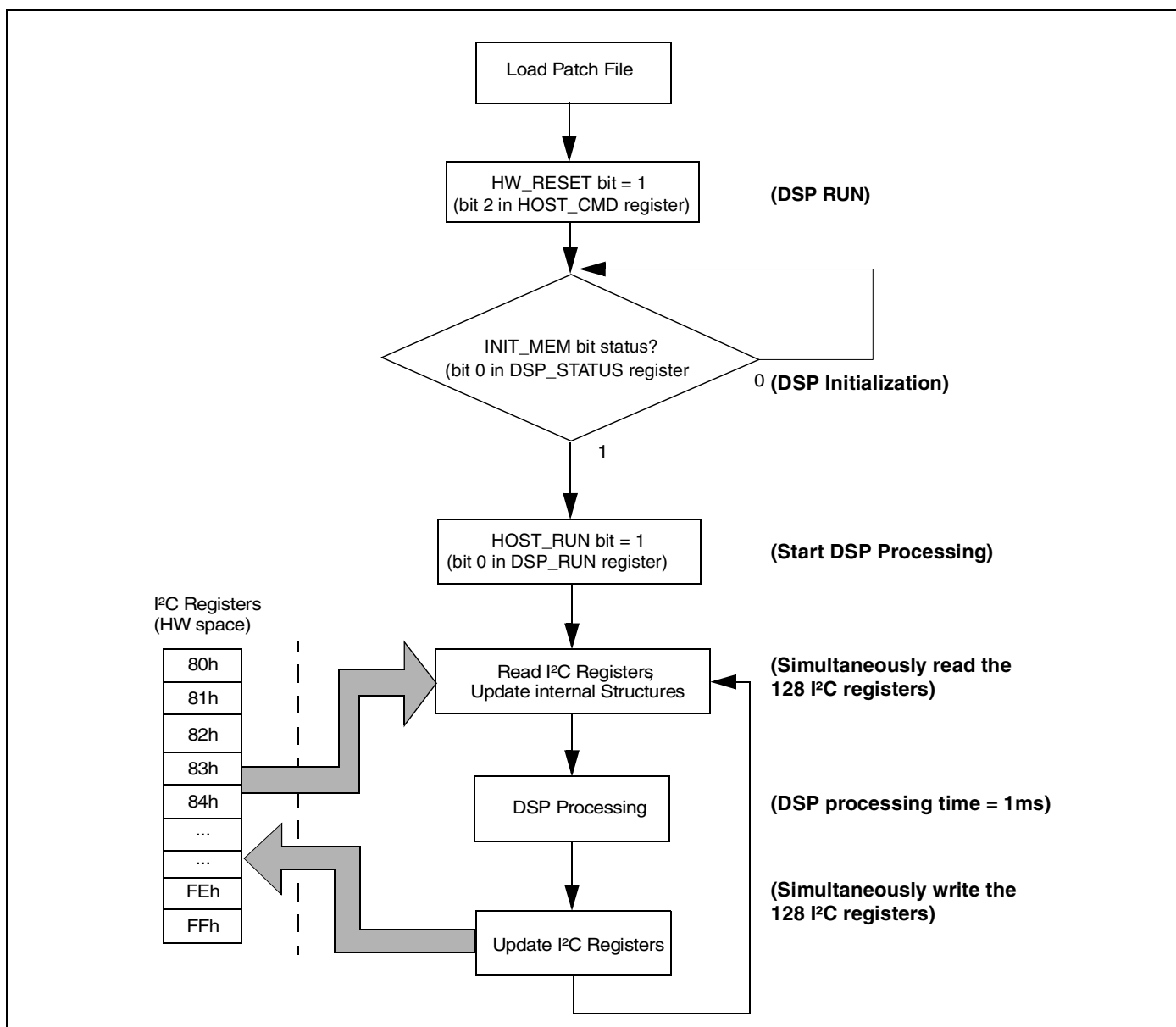
Figure 30: Simplified DSP Processing Flow
