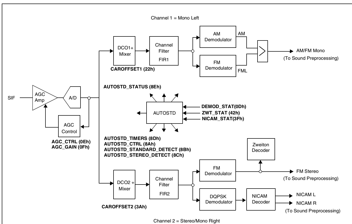
Figure 10: Demodulator Block Diagram
