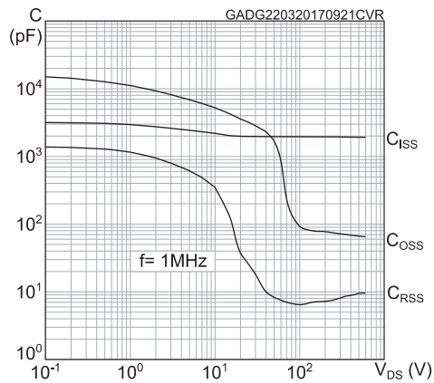
Figure 10: Capacitance variations
