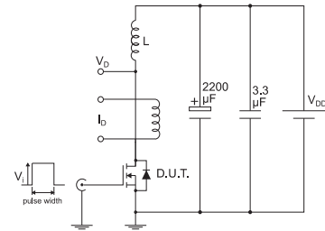
Figure 19: Unclamped inductive load test circuit
