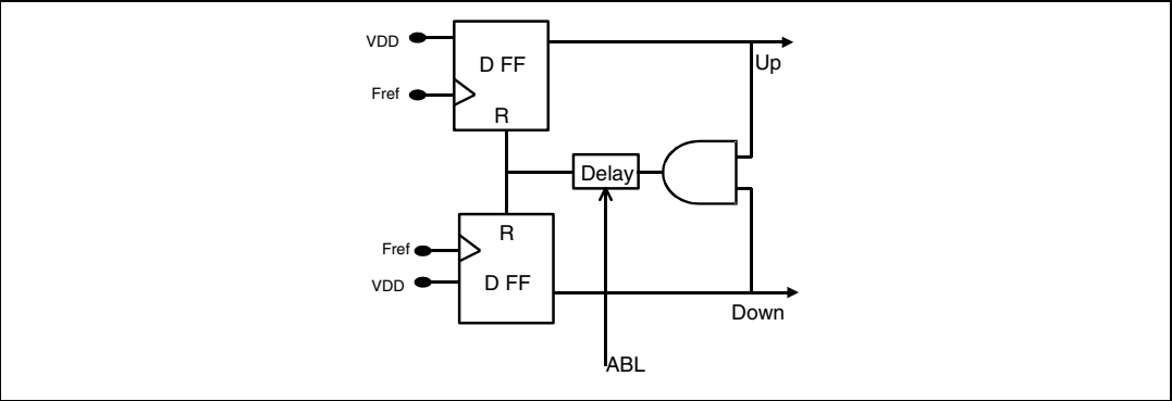
Figure 17. PFD diagram
