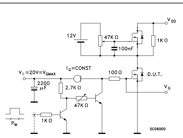
Figure 22. Gate charge test circuit
