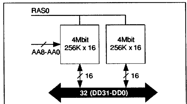
Figure 10 : 16-Mbit EDO DRAM Configuration
