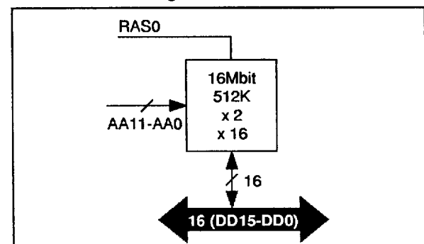
Figure 11 : 16-Mbit Synchronous DRAM Configuration
