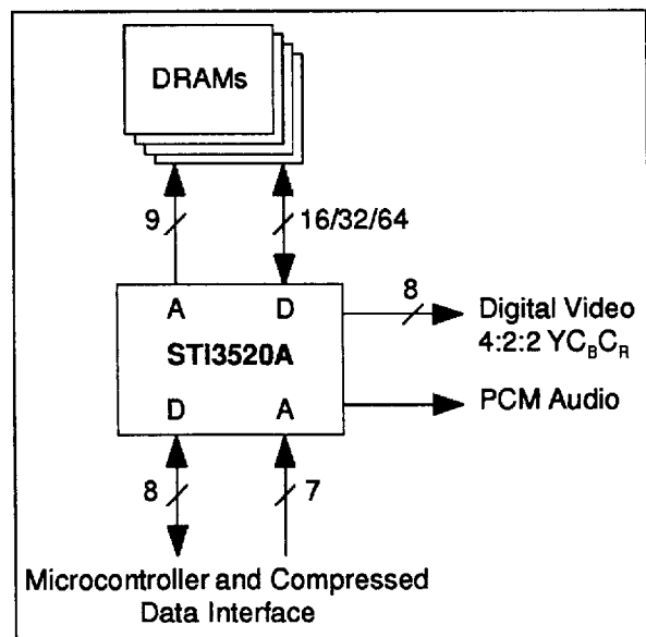
Figure 5 : Decoder System
