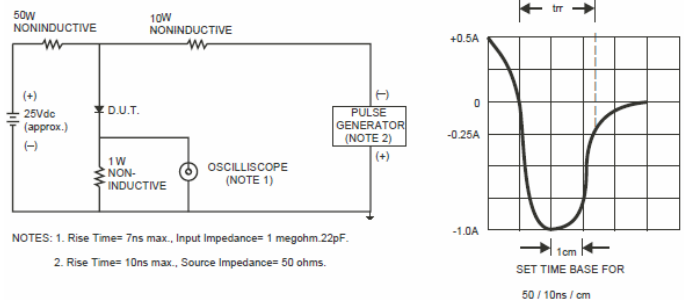
FIG. 6-Reverse Recovery Time Characteristic and Test Circuit
