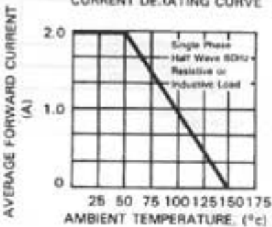
FIG. 5 - TYPICAL FORWARD CURRENT DERATING CURVE
