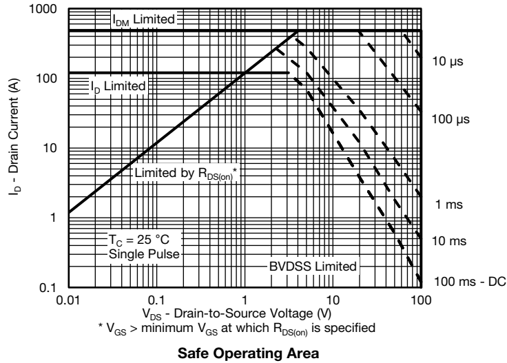
Safe Operating Area
