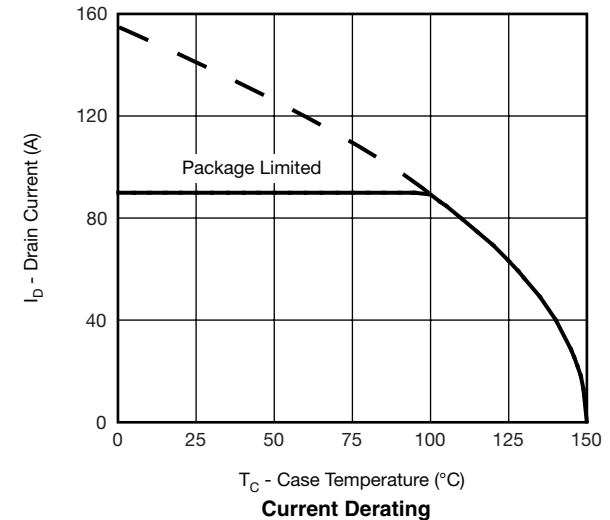
Current Derating
