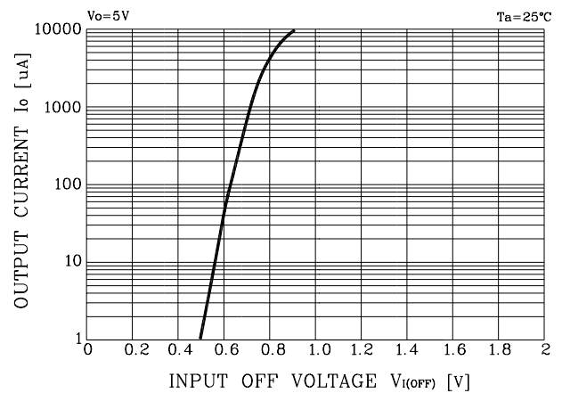
Fig. 2 I_O - V_{I(OFF)}
