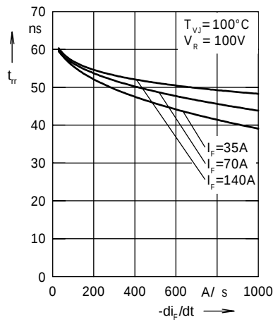
Fig. 5 Typ. recovery time t_{rr} versus -di_F/dt
