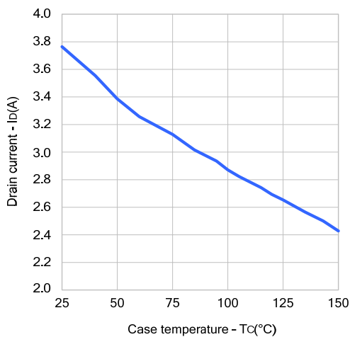
Figure 5. Drain Current vs. Case Temperature
