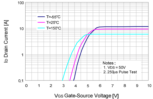
Figure 2. Transfer Characteristics
