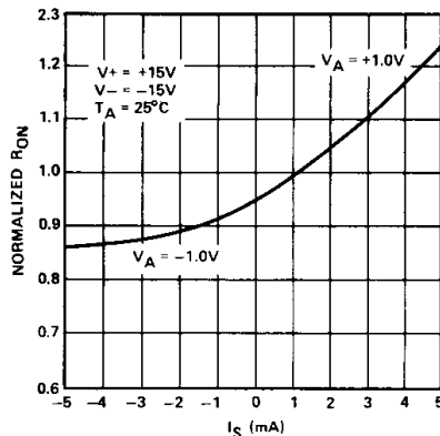
NORMALIZED R_{ON} vs SWITCH CURRENT ( I_S )
