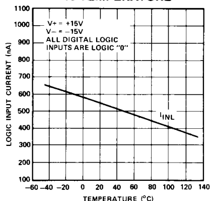
DIGITAL INPUT CURRENT I_{INL} vs TEMPERATURE
