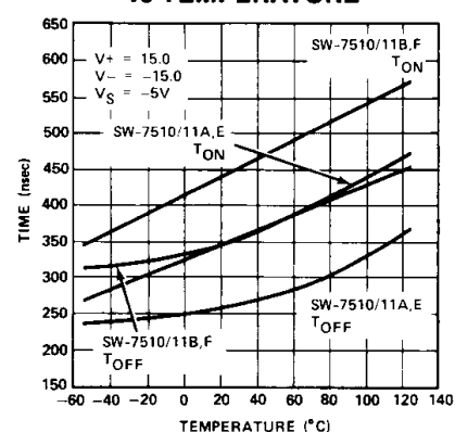
SWITCHING TIMES vs TEMPERATURE
