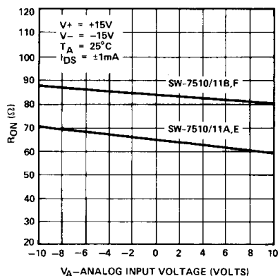
"ON" RESISTANCE ( R_{ON} ) vs ANALOG VOLTAGE ( V_A )
