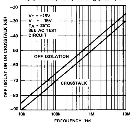
CROSSTALK AND "OFF" ISOLATION vs FREQUENCY
