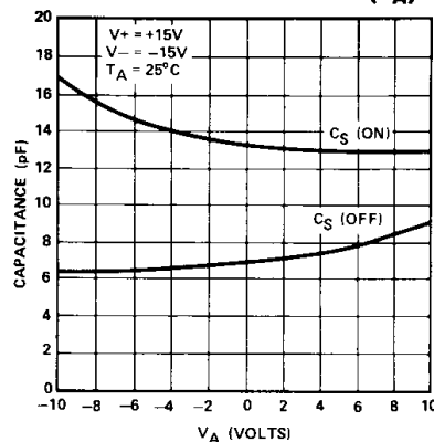
SWITCH CAPACITANCES vs ANALOG VOLTAGE ( V_A )
