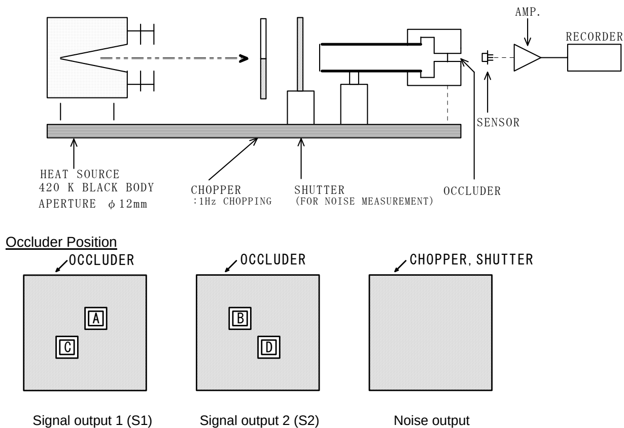
Fig. 2 : Test Set-up Block Diagram
