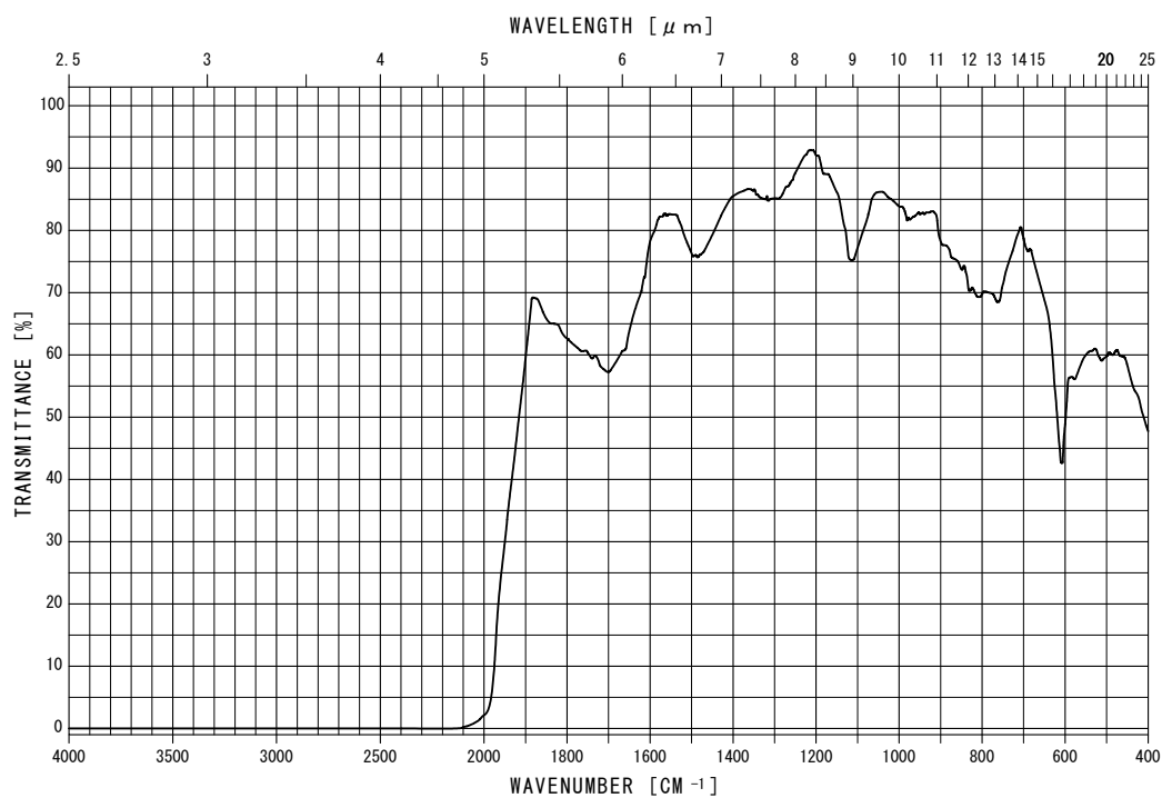
Fig. 4 : Typical Transmission Characteristics of Filter
