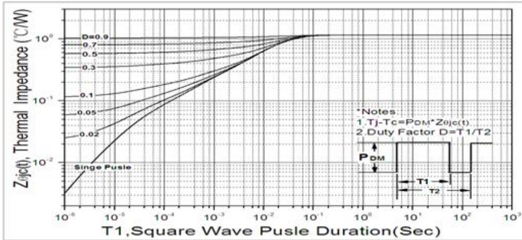
Fig. 17. Transient thermal response curve(TO-251N)
