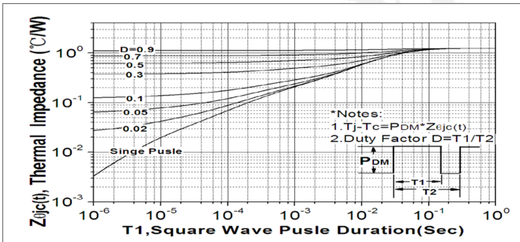
Fig. 18. Transient thermal response curve(TO-252)
