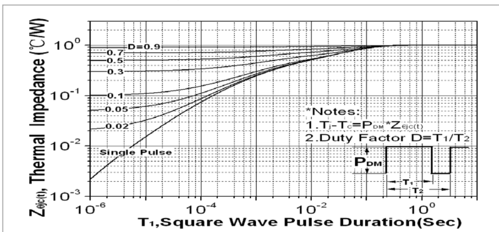
Fig. 19. Transient thermal response curve(TO-262)
