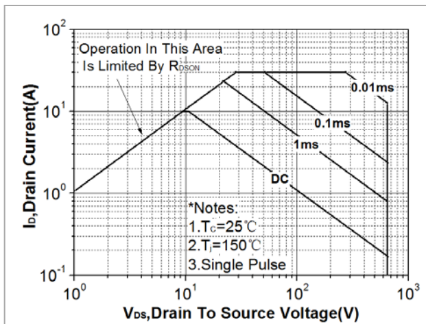
Fig. 11. Maximum safe operating area(TO-251N)
