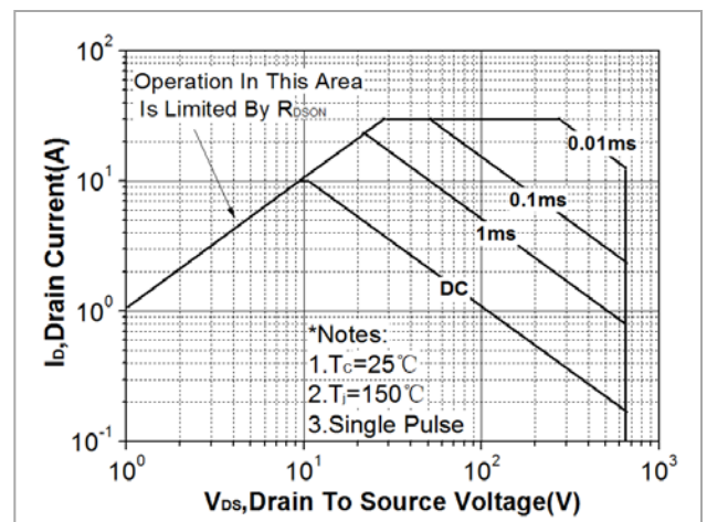
Fig. 12. Maximum safe operating area(TO-252)
