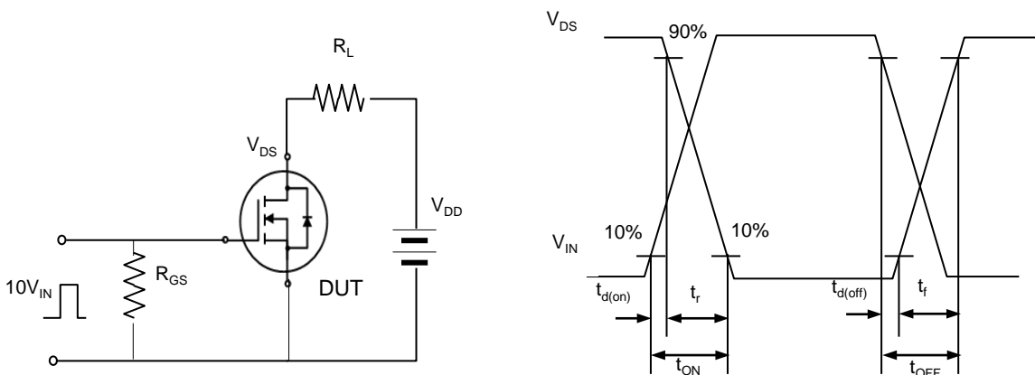
Fig. 22. Switching time test circuit & waveform
