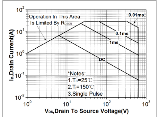
Fig. 14. Maximum safe operating area(TO-220SF)
