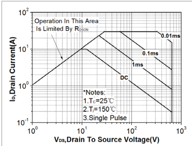
Fig. 13. Maximum safe operating area(TO-262)
