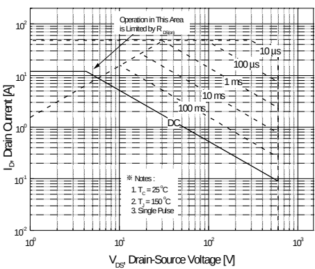
Fig. 10. Maximum safe operating area (TO-220F)
