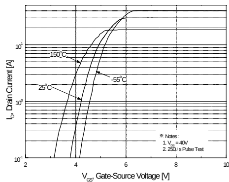
Fig. 2. Transfer characteristics
