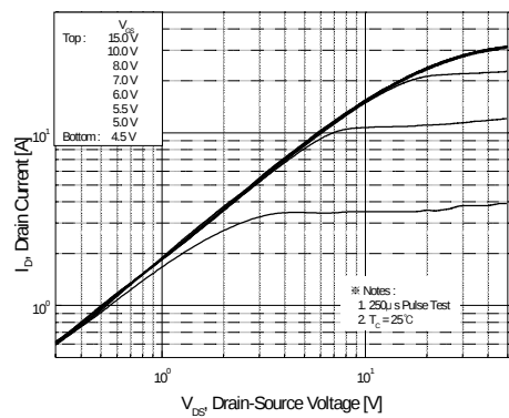
Fig. 1. On-state characteristics
