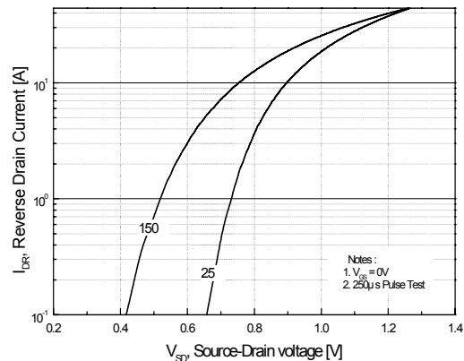
Fig. 4. On state current vs. diode forward voltage
