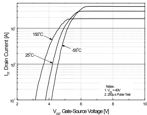
Fig. 2. Transfer characteristics
