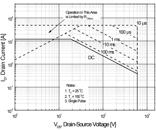
Fig. 10. Maximum safe operating area (TO-220F)
