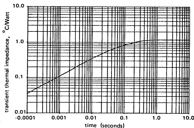
Figure 4 Transient thermal impedance, junction to case
