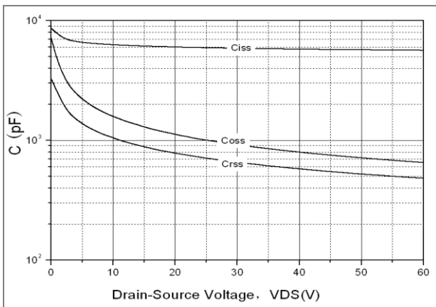
Fig. 9. Capacitance Characteristics
